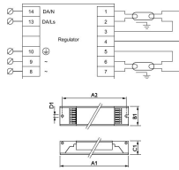
Specifications Philips HF-Ri TD 2 28-54 TL5 E+ 195-240V
