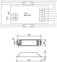
Specifications Philips Essential HF-E Ballast 1/2 55-58 W for TL5 - TL-D
